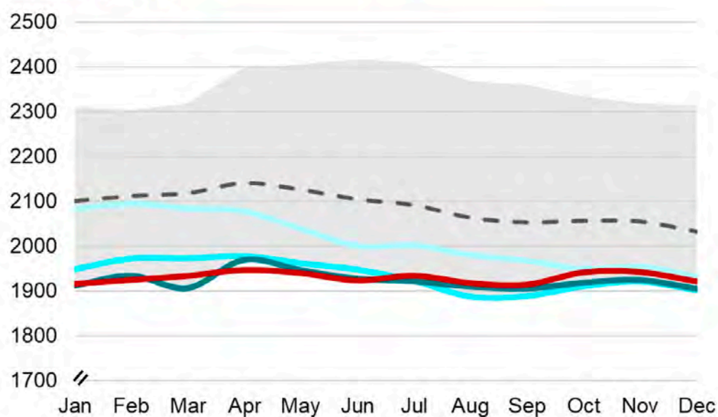
Crude Oil Closing Inventories (33 Countries)
