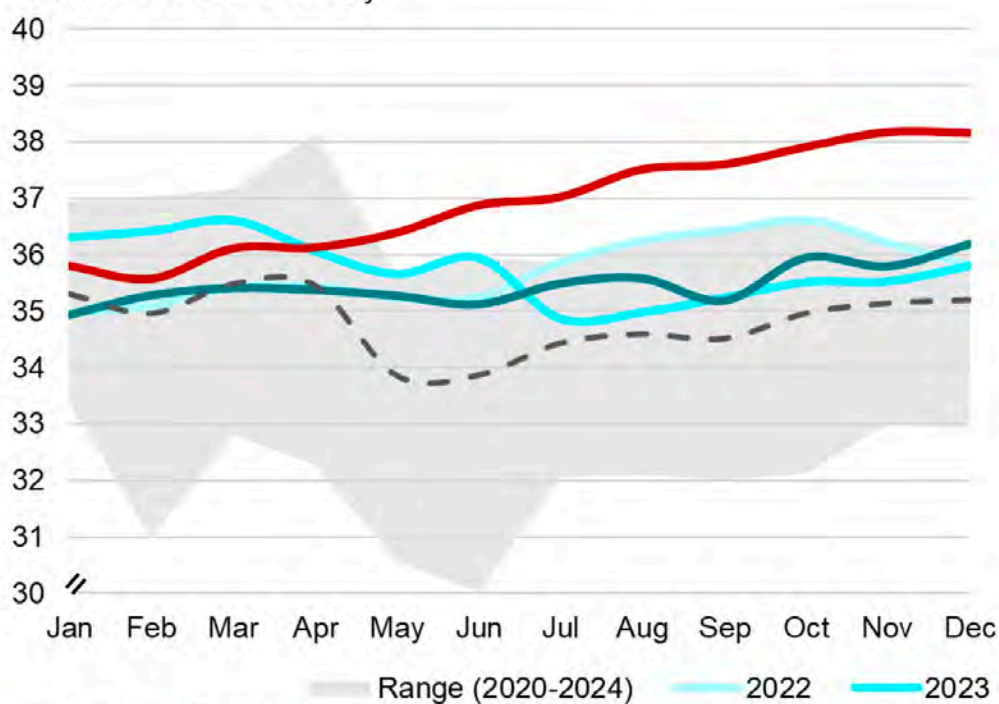
Crude Oil Production (28 Countries)
